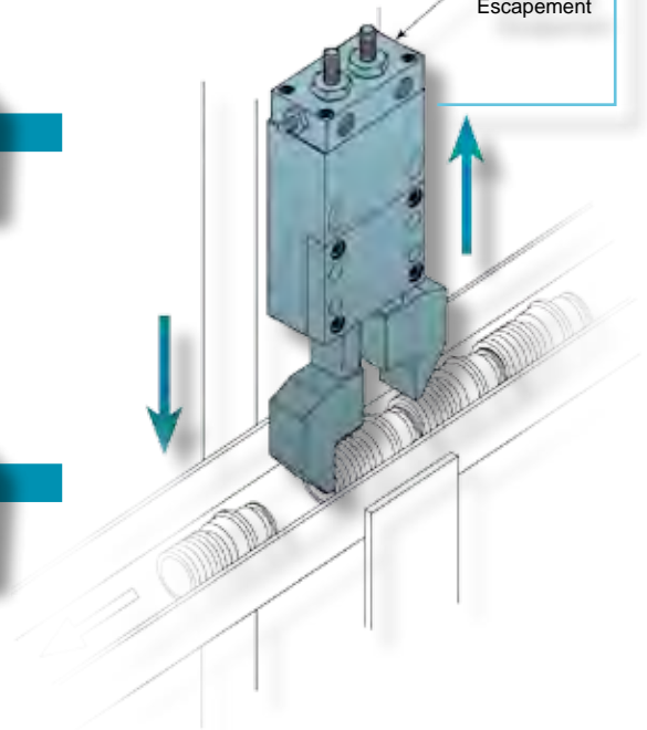
Series 160 Escapement
